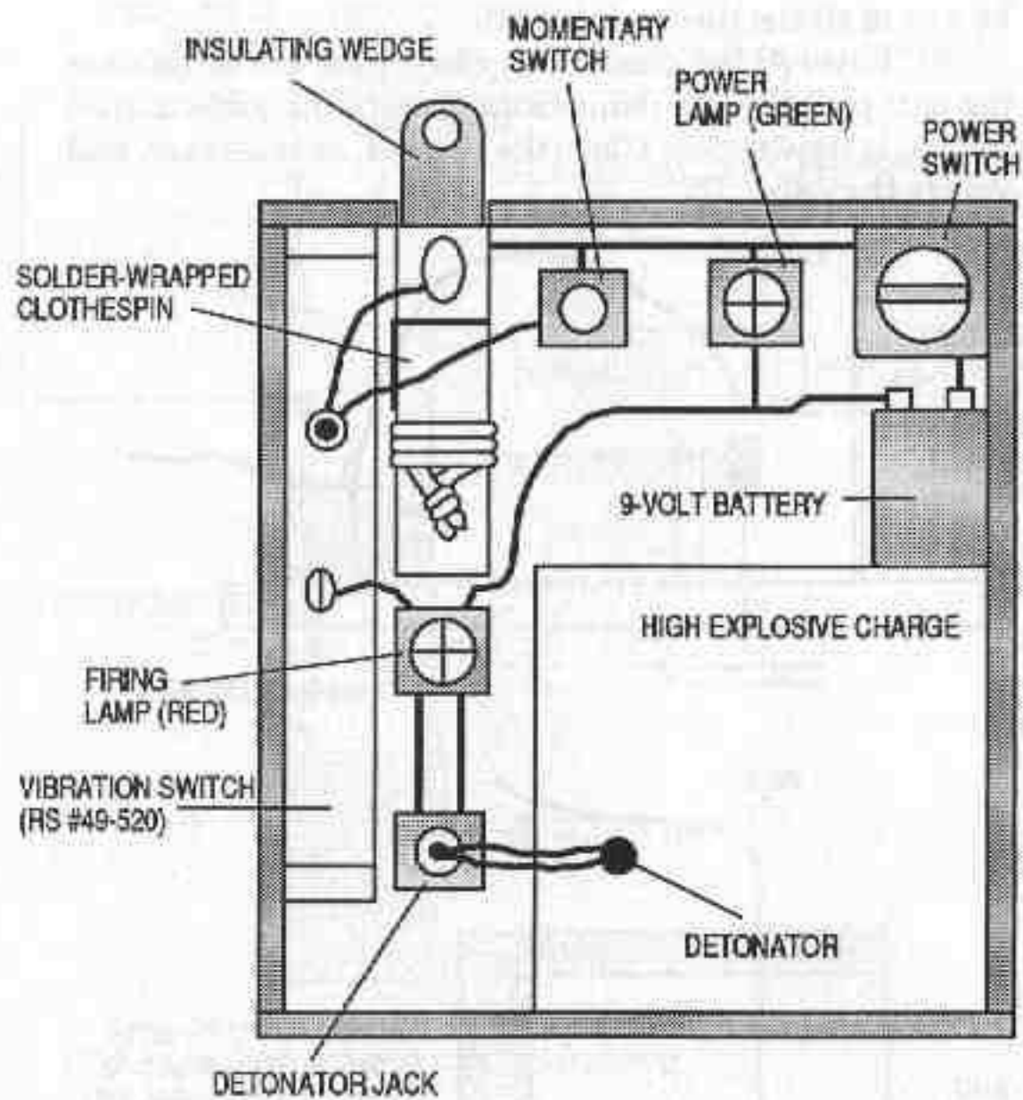
Antidisturbance mine.
