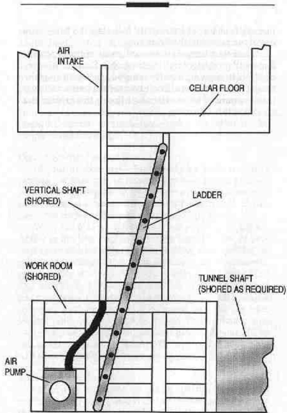
Tunnel entrance (not to scale—exaggerated for clarity).
