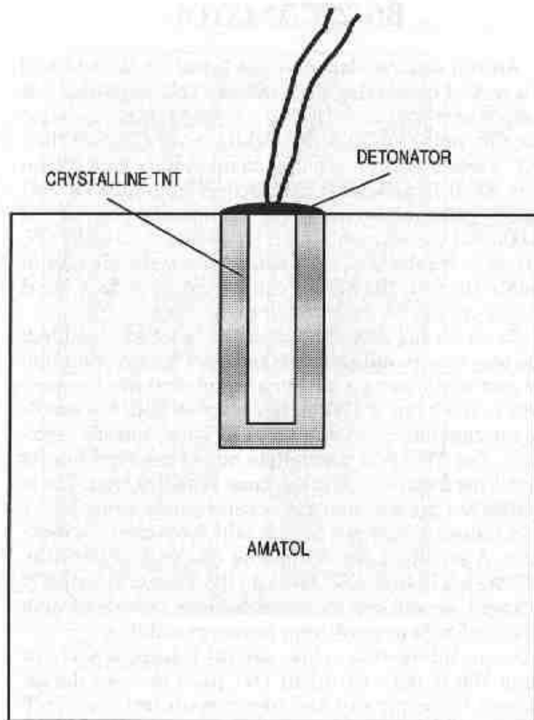
80/20 amatol demolition block.
