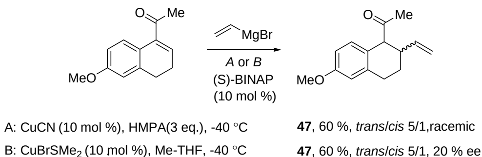
Scheme 5.2.8. Enantioselective conjugate addition by copper catalyst.
