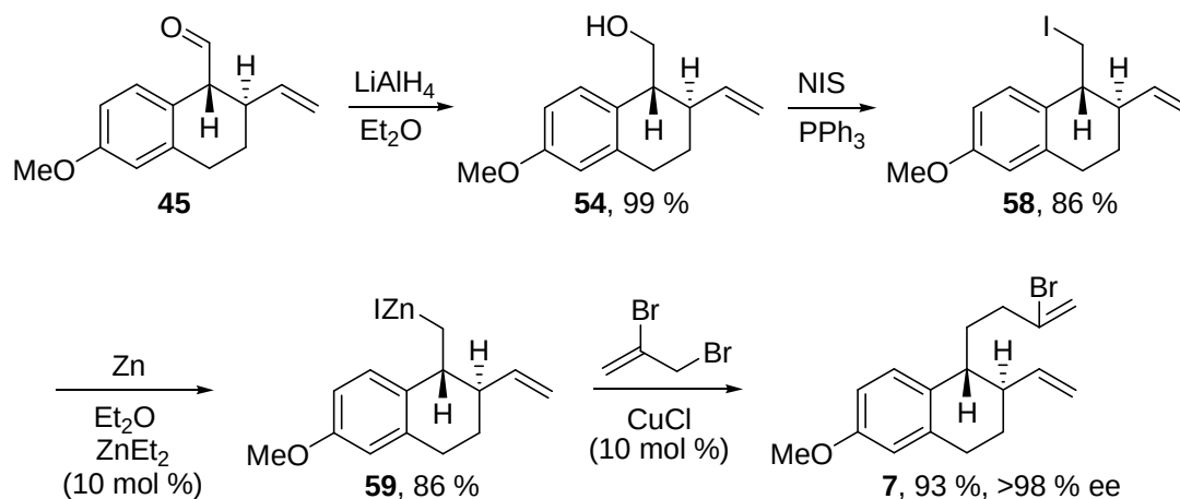
Scheme 5.2.13. Synthesis of chiral bromodiene 7 .
