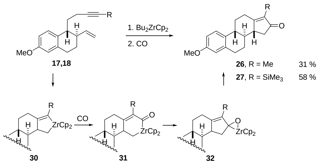
Scheme 5.1.14. Negishi's cyclocarbonylation.
