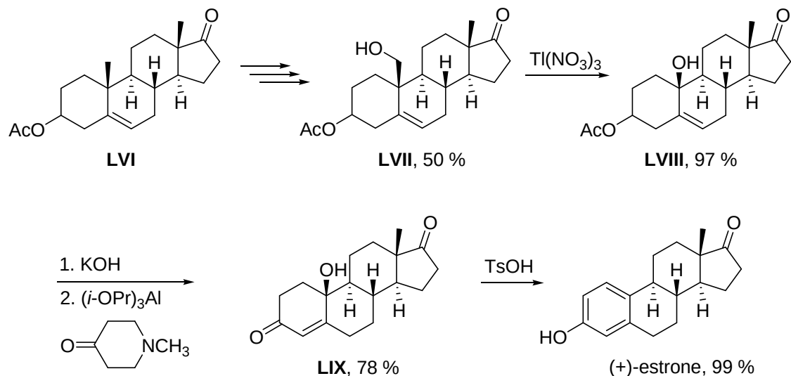
Scheme 3.8.3 Kočovský's synthesis of (+)-estrone.
