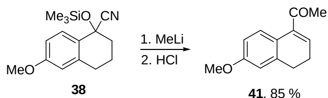
Scheme 5.2.3. Preparation of conjugated ketone 41 .
