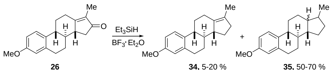
Scheme 5.1.17. Reduction of the 26 with Et 3 SiH.
