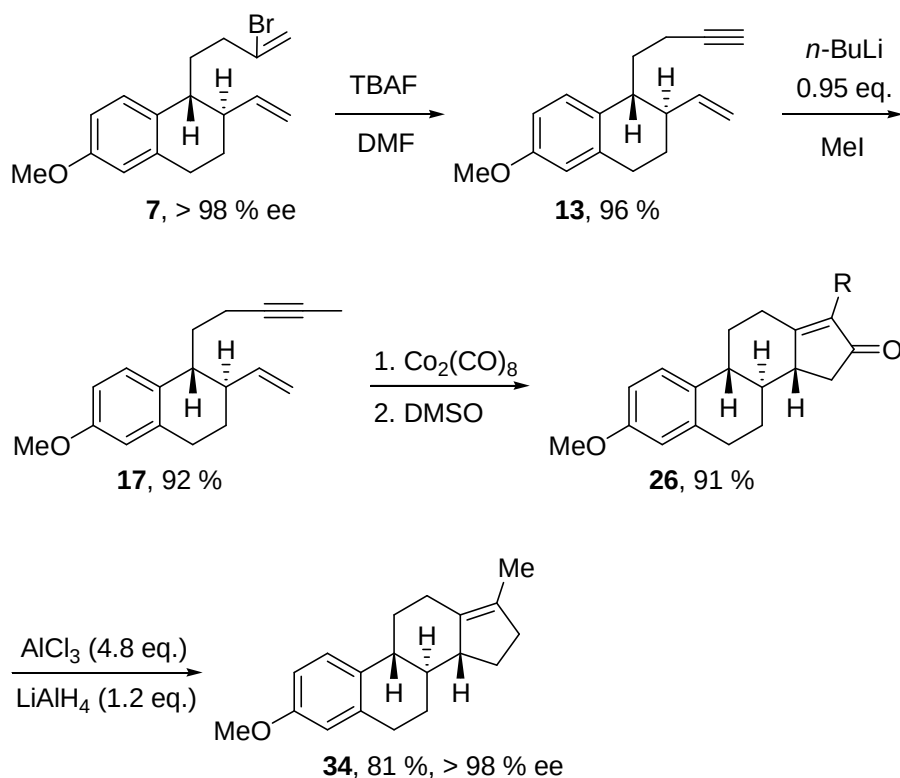
Scheme 5.2.14. Synthesis of chiral 17-methylestratetraene 34 .
