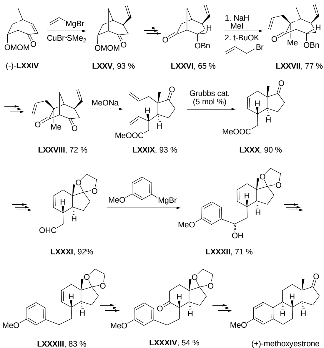
Scheme 3.9.4
