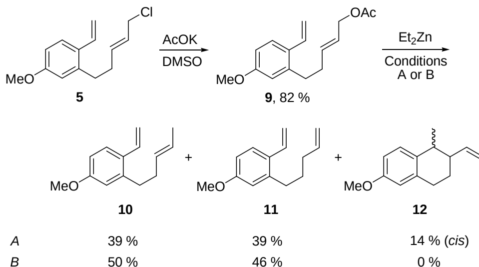
Scheme 5.1.5. Palladium catalyzed metallo-ene cyclization of 9 .
