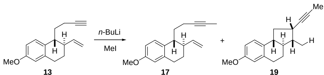
Scheme 5.1.8. Methylation of enyne 13 .
