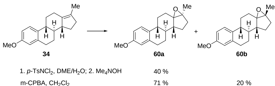
Scheme 5.2.15. Epoxidation of 34 .
