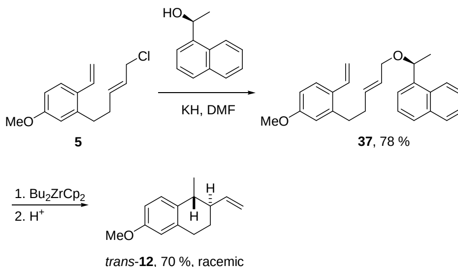
Scheme 5.2.1. Zirconocene mediated cyclization of chiral ether 37 .
