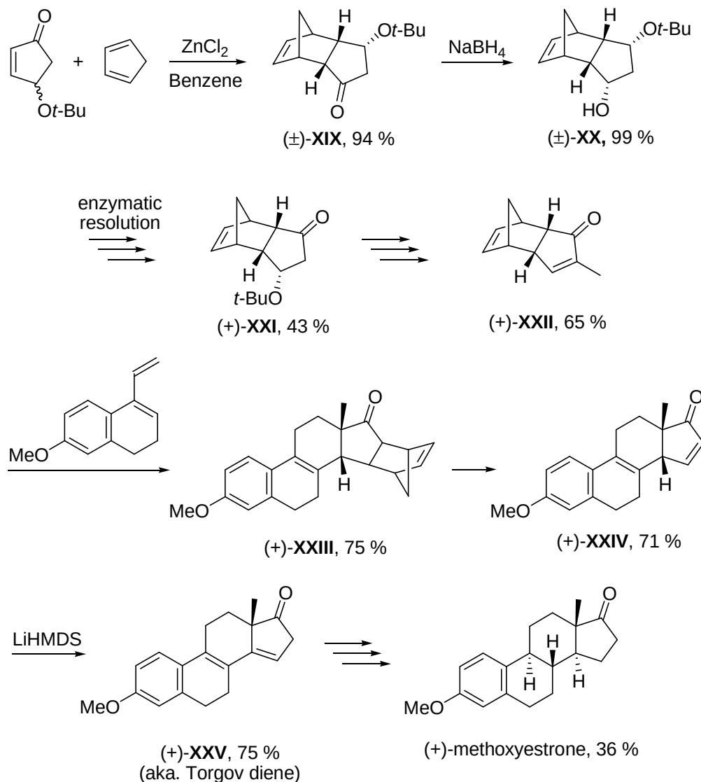
Scheme 3.3.1 Ogasawara's synthesis.
