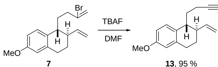
Scheme 5.1.6. Dehydrobromination of bromodiene 7 .
