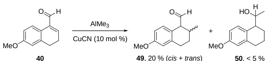
Scheme 5.2.7. Conjugate addition of \text{AlMe}_3 .
