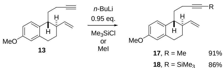
Scheme 5.1.10. Methylation and silylation of enyne 13 .
