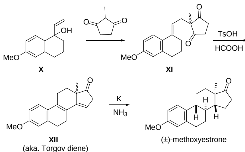
Scheme 3.2.2 Windholz's synthesis.
