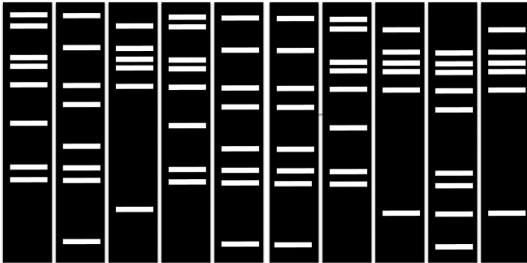
Figure 39-8 Pulsed-field gel electrophoresis. Pulsed-field gel electrophoresis (PFGE) is used for genotyping prokaryotes, and it was the gold standard for epidemiological studies until DNA sequencing became readily available. Large DNA fragments, 20 kb to >1 Mb, are separated by gel electrophoresis utilizing pulsed electrical fields. These large fragments are usually generated by digesting the DNA with rarely cutting restriction endonucleases, in general enzymes that recognize eight or more nucleotide bases. This technique is used because DNA fragments larger than 30 to 50 kb run at the same rate in standard gel electrophoresis. In contrast to the standard gel electrophoresis method, in which the voltage is constantly running in one direction, for PFGE the voltage is periodically switched among three directions. One direction is the central axis of the gel, and the other two are at a 60° angle on either side. This periodic change in field direction allows various lengths of DNA to change at different rates. Larger fragments of DNA will realign more slowly than smaller pieces when the field direction is changed. The separated fragments can be visualized, for example, by using ethidium bromide. This figure shows that control 1 is related to isolates 3 and 6 while control 2 is related to isolates 2 and 7.
