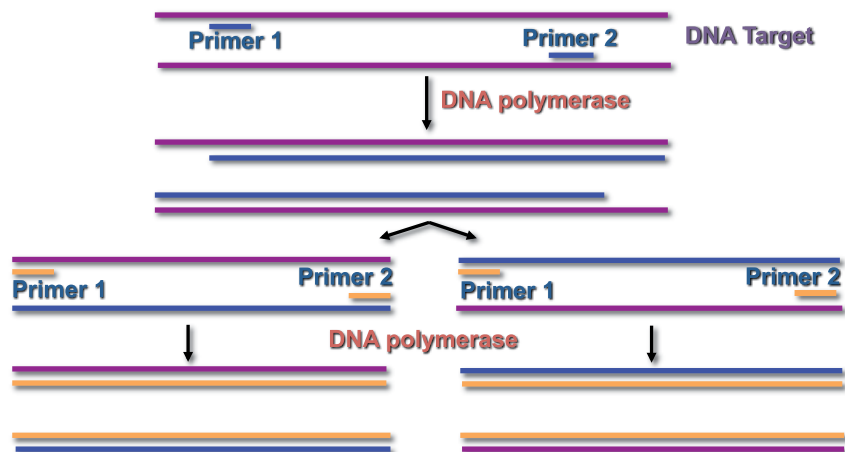
Figure 39-13 PCR. In PCR amplification, in addition to the target dsDNA, two oligonucleotides (primers), a heat-stable DNA polymerase, and the four dNTPs are added in a buffer solution. The two primers are complementary to opposite strands of the target and are usually at a distance of 100 to 500 bp from each other. The reaction starts by increasing the temperature to approximately 95°C to denature the target dsDNA. This is followed by cooling to approximately 60 to 65°C to allow the primers to anneal to the target DNA. The DNA polymerase then initiates the extension of the primers, producing new dsDNA copies. Under ideal conditions, the number of target sequences doubles each cycle. In a 100% efficient reaction, a 10^6 -fold amplification occurs after 20 cycles and a 10^9 -fold amplification is obtained after 30 cycles. The amplified DNA can be detected by various methods, including the use of fluorescent dyes, such as ethidium bromide, after running a gel or by using labeled oligonucleotides complementary to the amplified target. Internal controls can be included in the reaction mixture to make sure that no inhibitory substances such as hemoglobin interfered with the amplification. Numerous commercial kits are available for the detection of pathogens using PCR.
