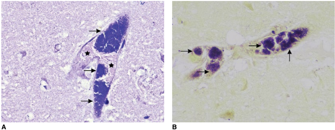
Figure 41-60 Septic cerebral embolism. (A) Brain section stained with H&E (objective magnification, ×50) showing intravascular (stars) bacterial emboli (arrows) from a patient who died of Staphylococcus aureus bacteremia. (B) Modified Brown and Hoppps (objective magnification, ×40) of the same tissue shows intravascular Gram-positive cocci in clusters (arrows).
